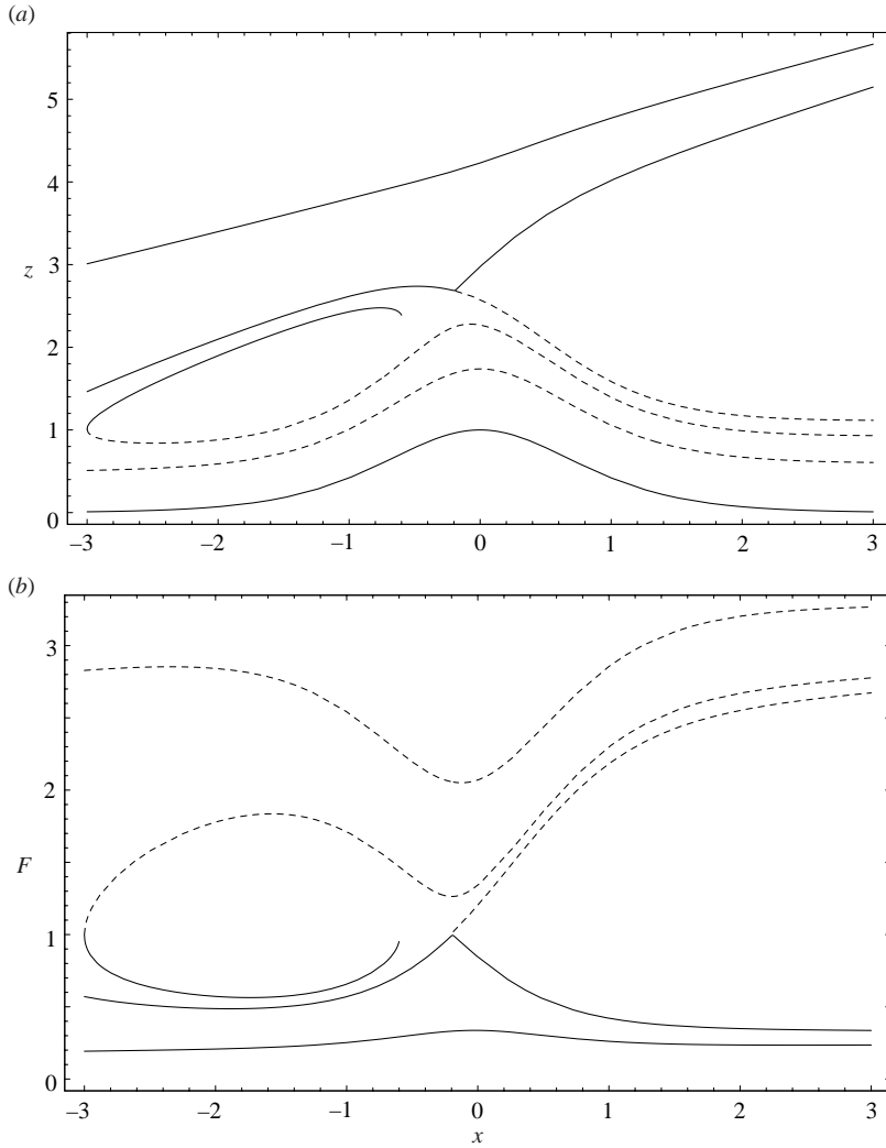
FIGURE 6. As figure 4 except that u_1 = 3 .
